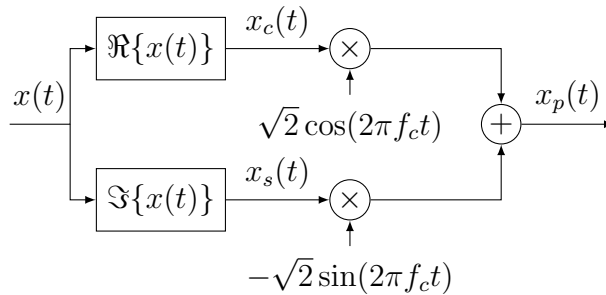
Figure 1.2: Conversion of a baseband signal to a passband signal.
